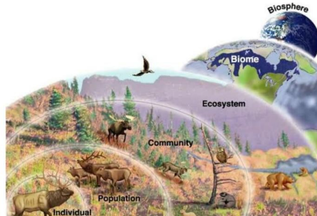
Fig: Levels of biological organization — individual, population, community, ecosystem, biome and biosphere.
