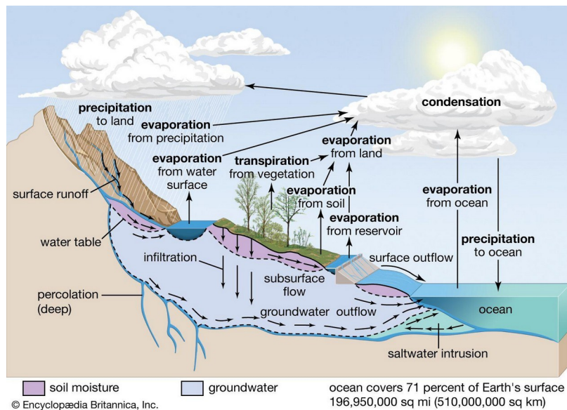
Fig: The Hydrologic (Water) Cycle.
