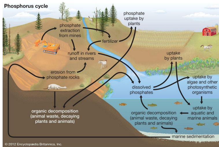
Fig: The Phosphorus Cycle.
