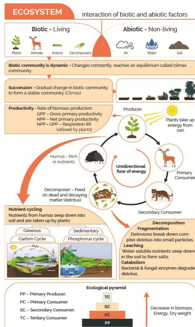
Fig: Interaction of biotic and abiotic factors in an ecosystem, showing productivity, nutrient cycling and the ecological pyramid.
