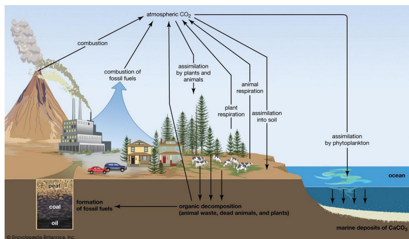
Fig: The Carbon Cycle.
