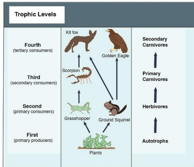
Fig: Trophic levels and food web — from primary producers to tertiary consumers.
