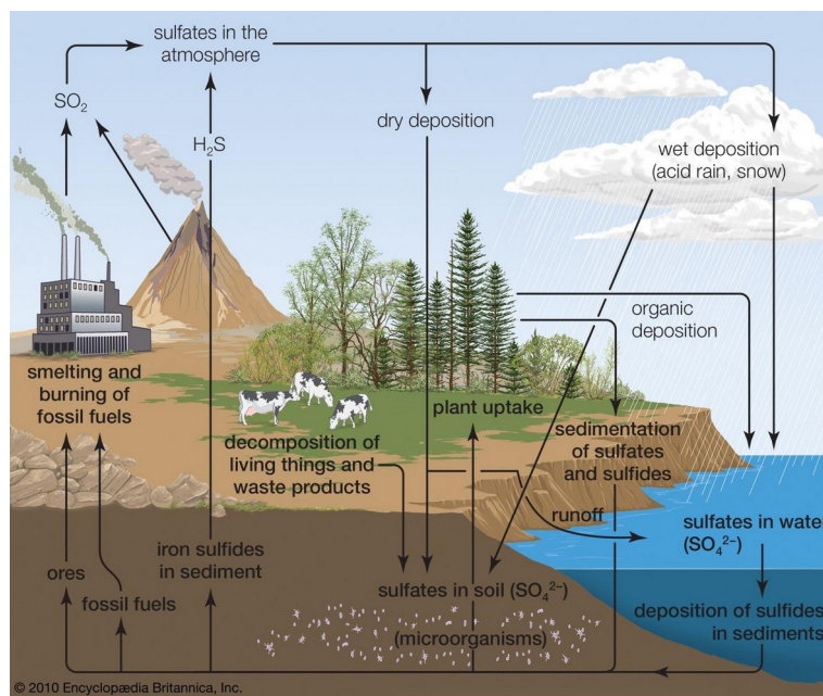
Fig: The Sulphur Cycle.
