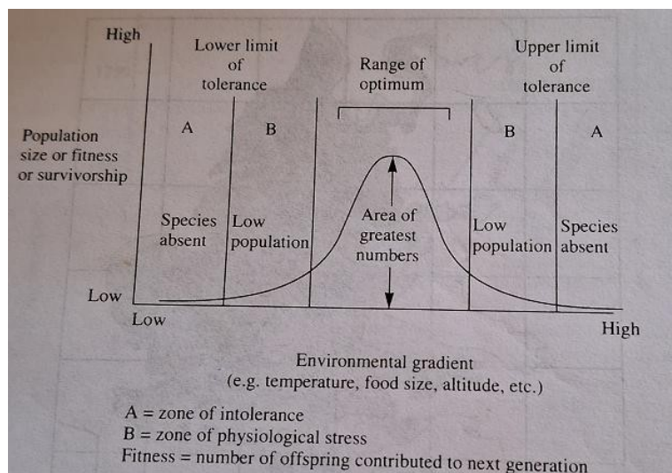
Fig: A schematic tolerance curve for a single species population existing on a single environmental gradient.
